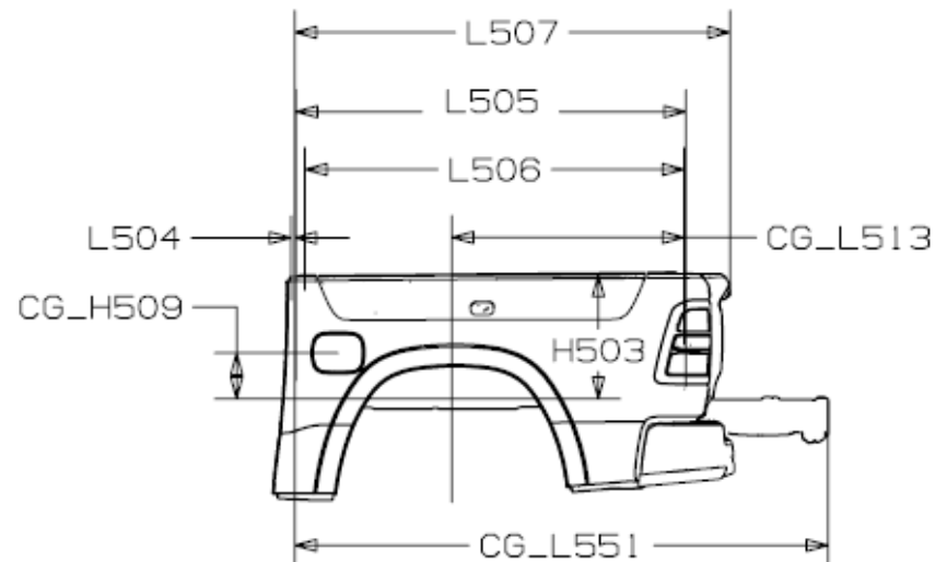
Ram 1500 (DT) 5' 7" Box Drawing (With RamBox)
