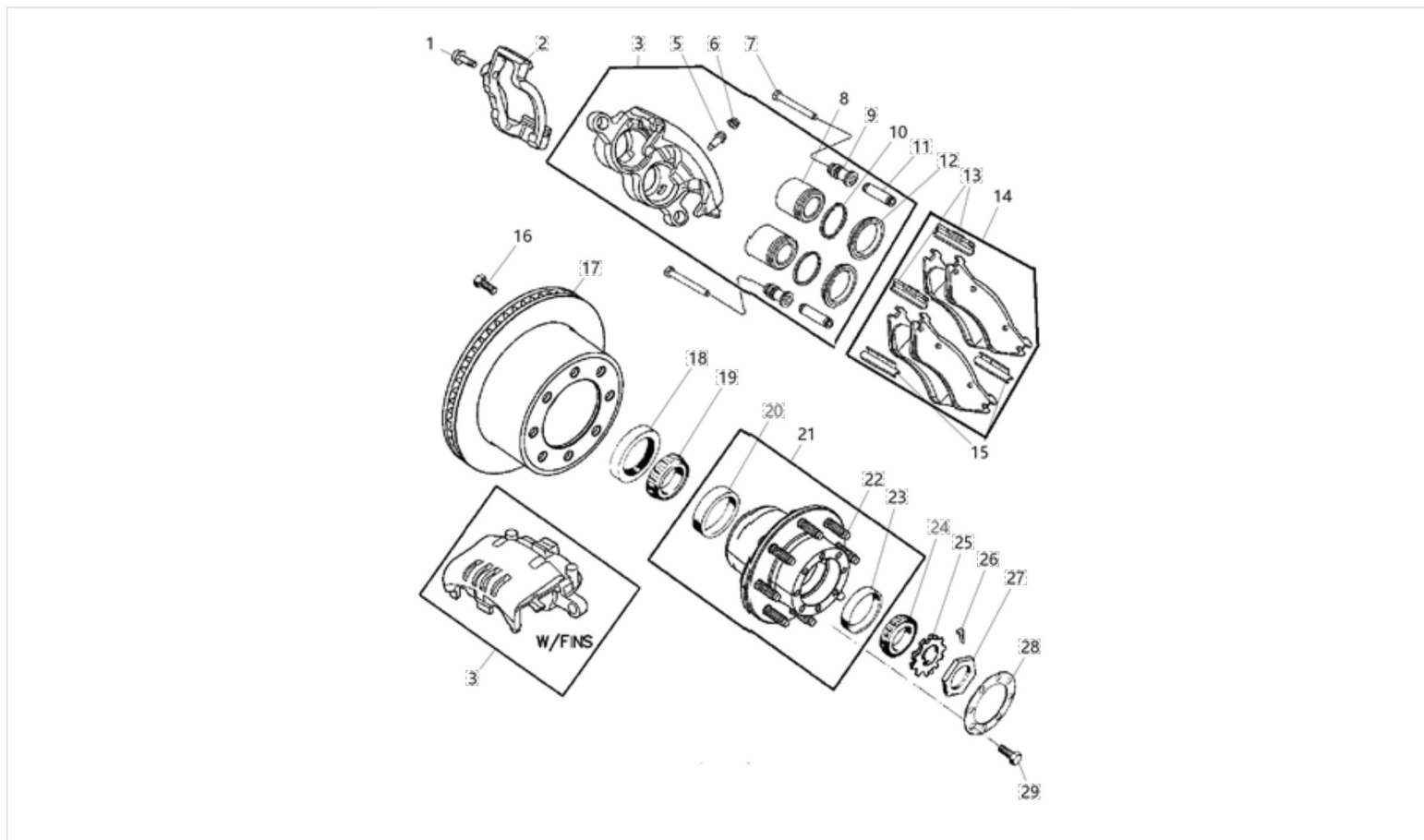
Diagram (2 of 2): Service Brakes Brakes,Rear,Disc,DR 2,3,7,8
