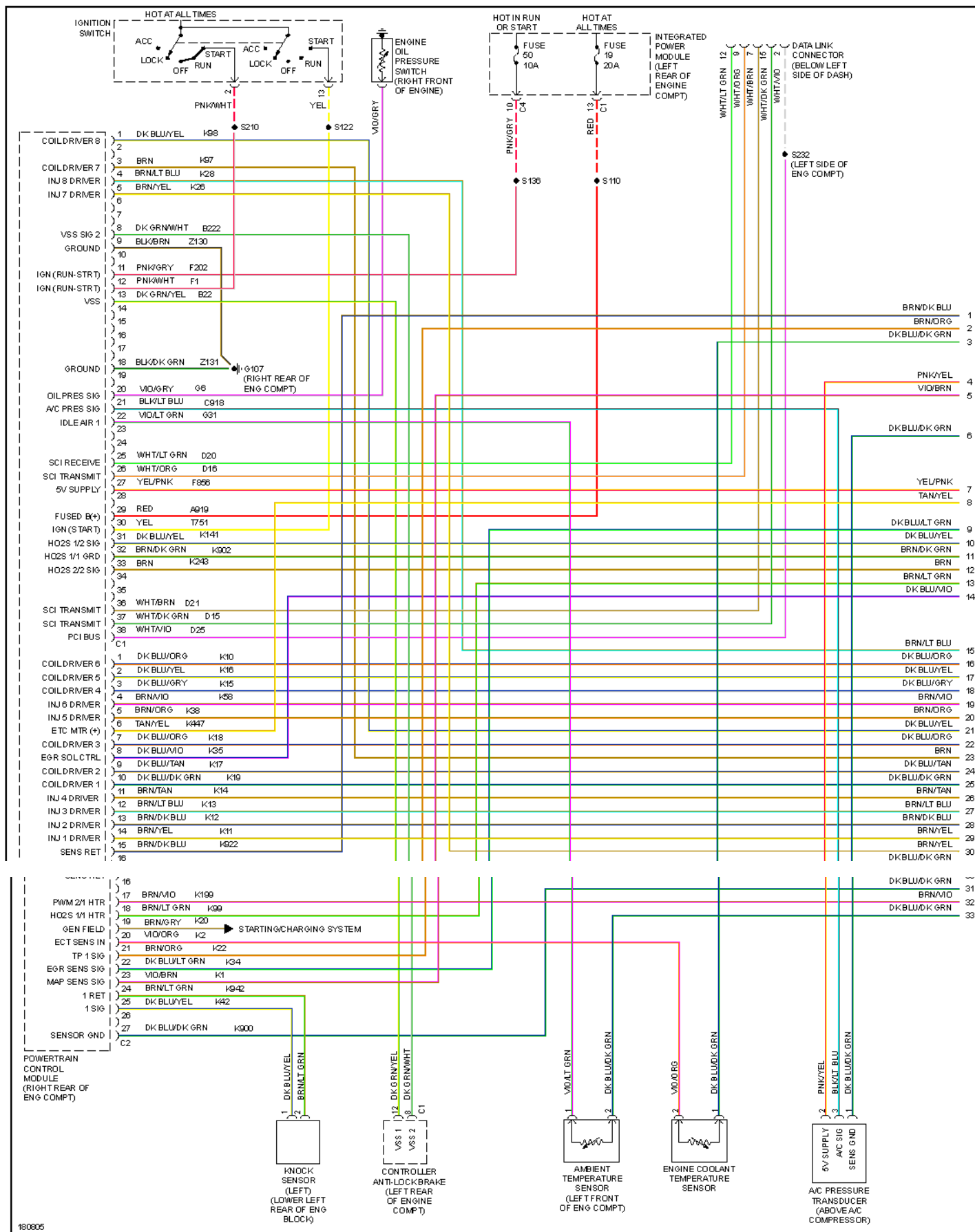
Fig. 24: 5.7L Engine Performance Circuit (1 of 5)
