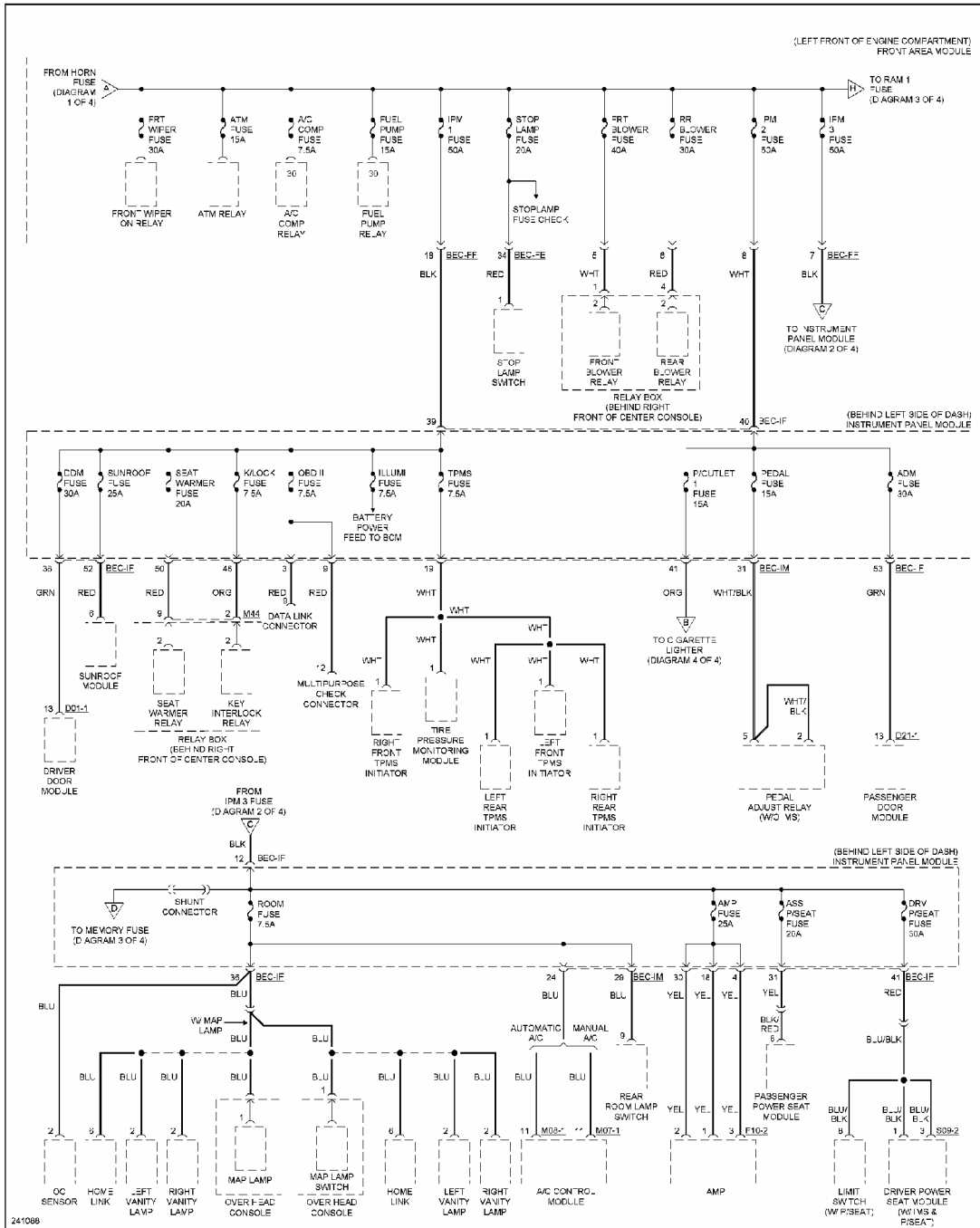
Fig. 51: Power Distribution Circuit (2 of 4)
